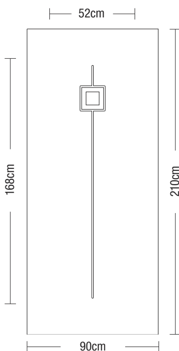
Panel dimensions
