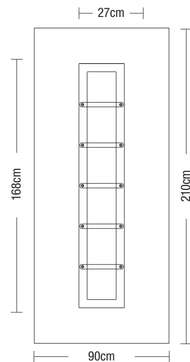
Panel dimensions
