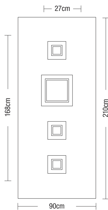
Panel dimensions
