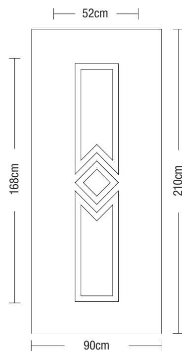
Panel dimensions
