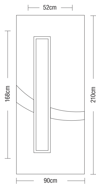
Panel dimensions
